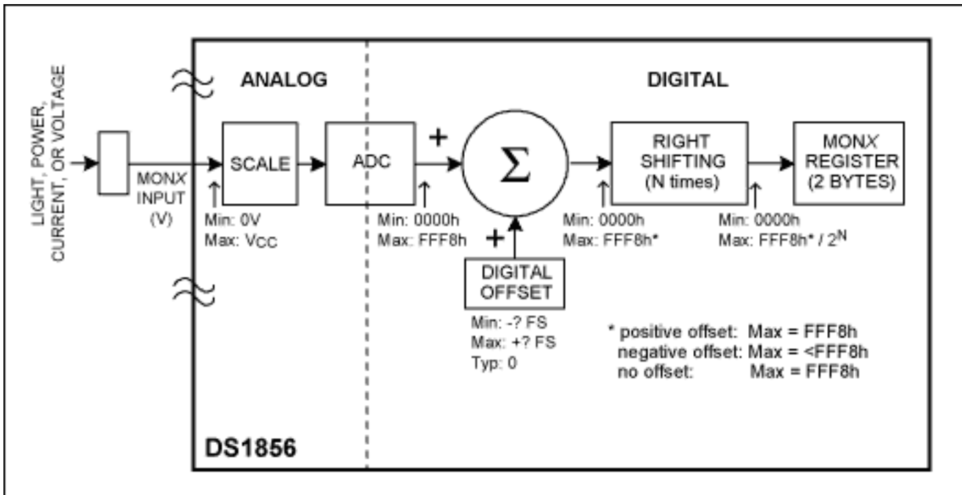
Figure 1. DS1856 MON Input Block Diagram
